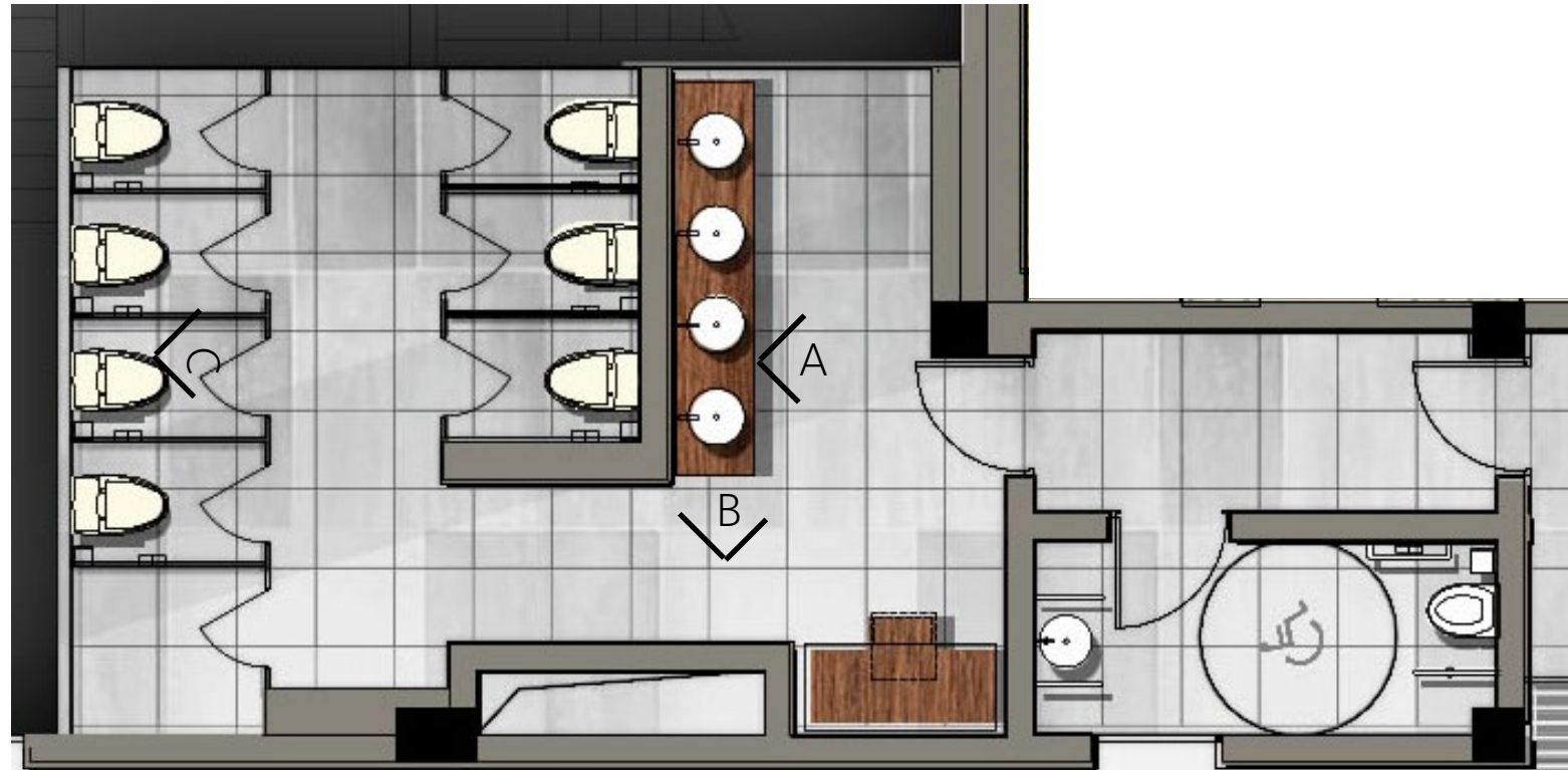
FEMALE TOILET & DISABLE TOILET
